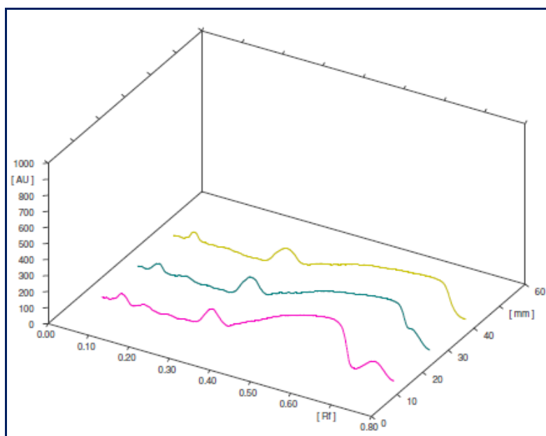
Fig 7: 3D chromatograms of all tracks at 540 nm after derivatization
