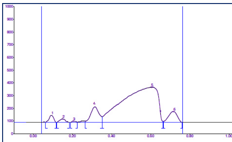
Fig 6: HPTLC finger print profile of chloroform extract of Milagathi chooranam at 540 nm
