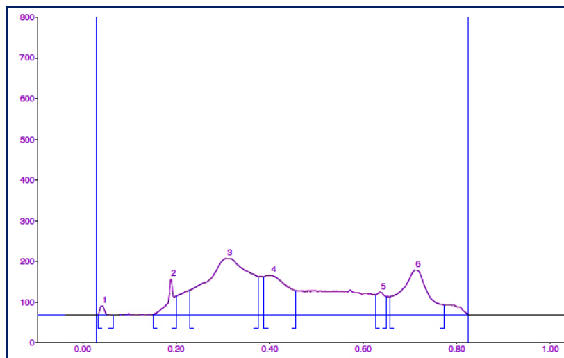
Fig 4: HPTLC finger print profile of chloroform extract of Milagathi chooranam at UV 366 nm
