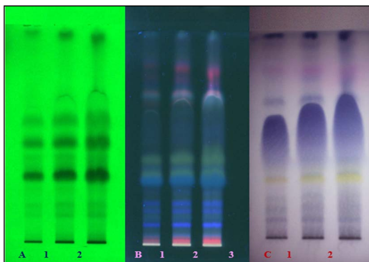
Fig 1: TLC photodocumentation of chloroform extract of Milagathi chooranam A.UV 254 nm; B.UV 366 nm; C. After derivatization; Track 1.5 \mu l; Track 2.10 \mu l; Track 3.15 \mu l
