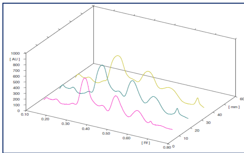
Fig 3: 3D chromatograms of all tracks at UV 254 nm
