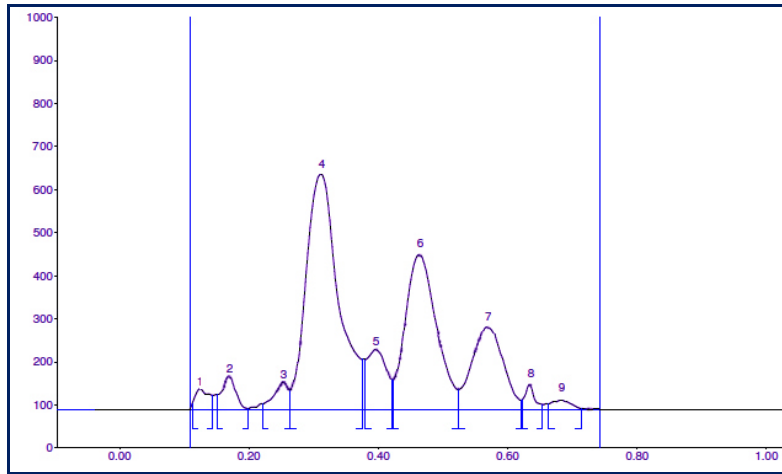
Fig 2: HPTLC finger print profile of chloroform extract of Milagathi chooranam at UV 254 nm
