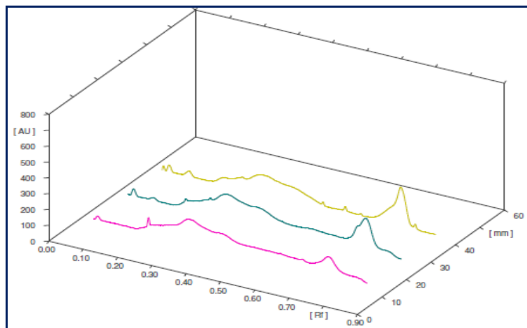
Fig 5: 3D chromatograms of all tracks at UV 366 nm
