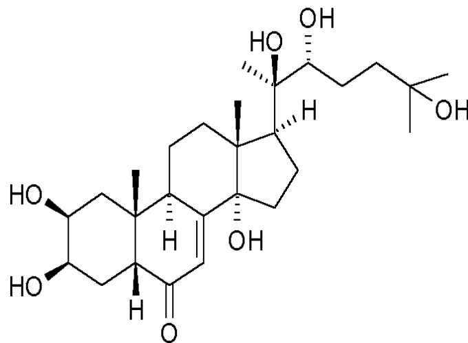
Fig 3: Structure of ecysterone (20- hydroxy eclyson)
